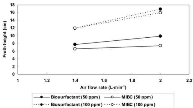
Fig. 2. Froth height as a function of air flow rate.
